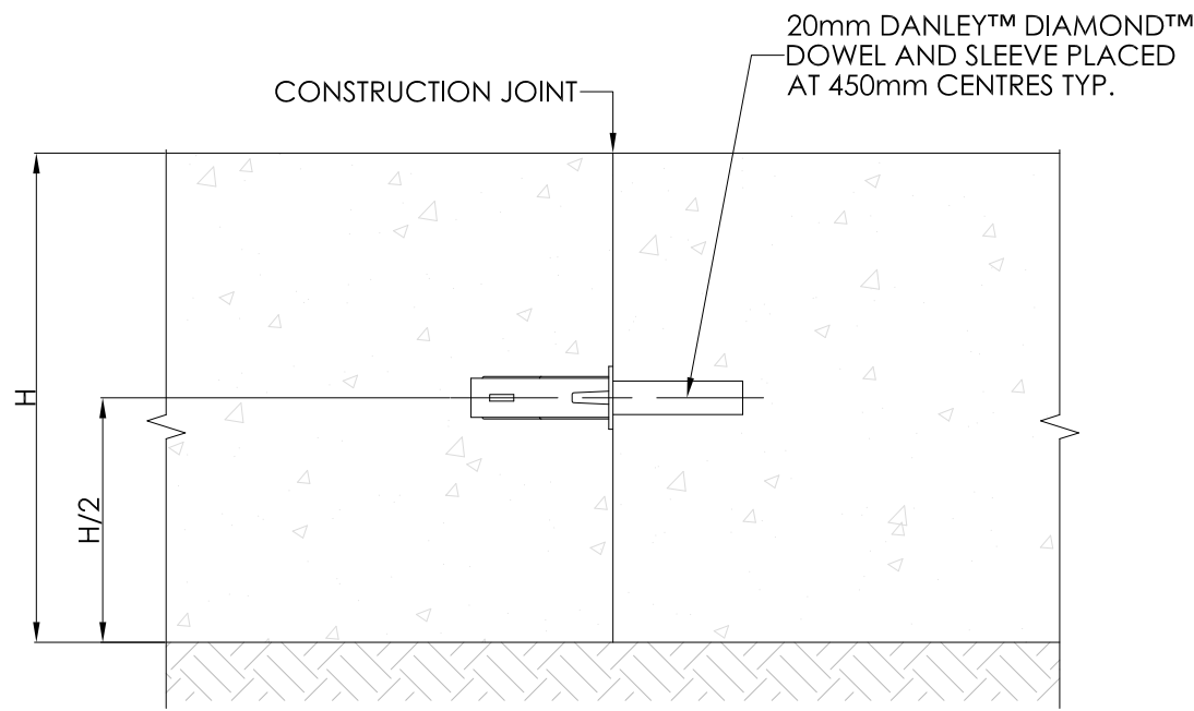
PLATE DOWEL JOINT (P.D.J.)
