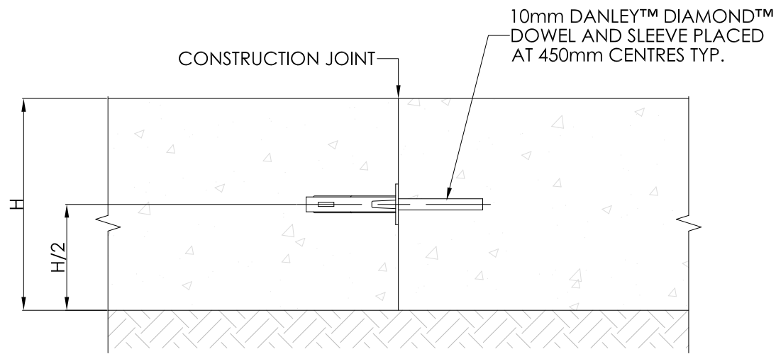
PLATE DOWEL JOINT (P.D.J.)
