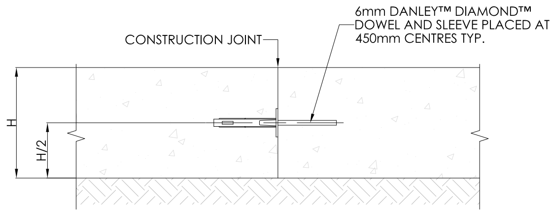
PLATE DOWEL JOINT (P.D.J.)
